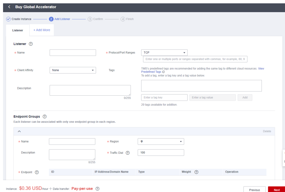
Figure 1-2 Adding a listener
