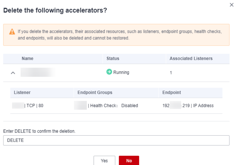
Figure 1-3 Deleting a global accelerator
